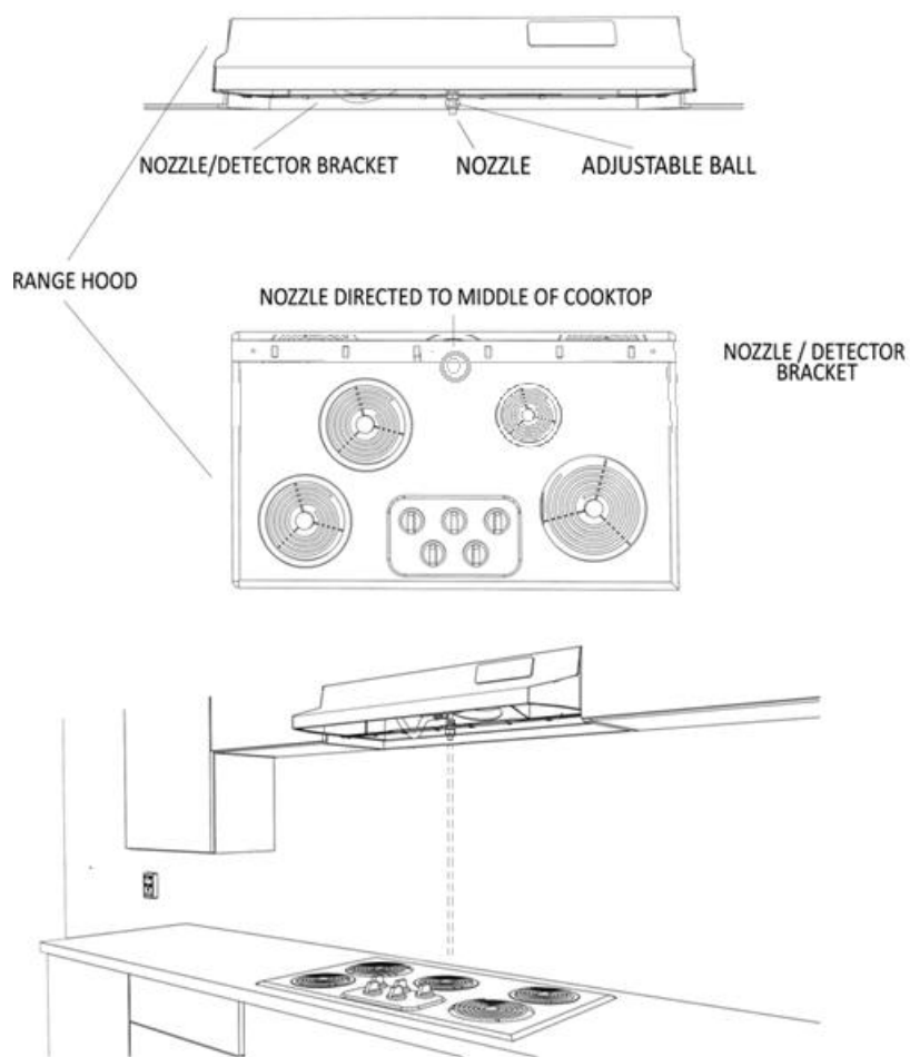
Illustration showing nozzle location
